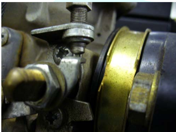
Figure 42a: Throttle idle screw clear of lever.
