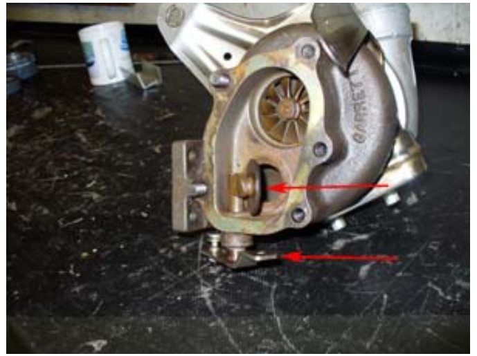
Figure 17: Inside of turbo showing waste gate and control lever
