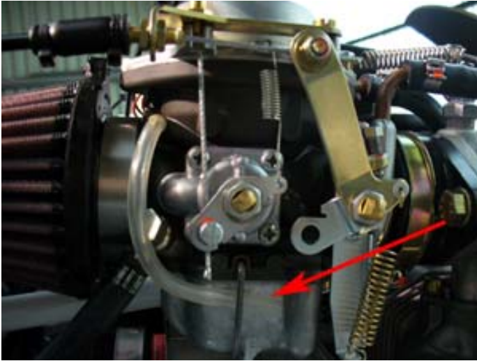
Figure 34: Correct carb overflow pipe vent arrangement and sprung open throttle system with correctly fitted choke levers.
