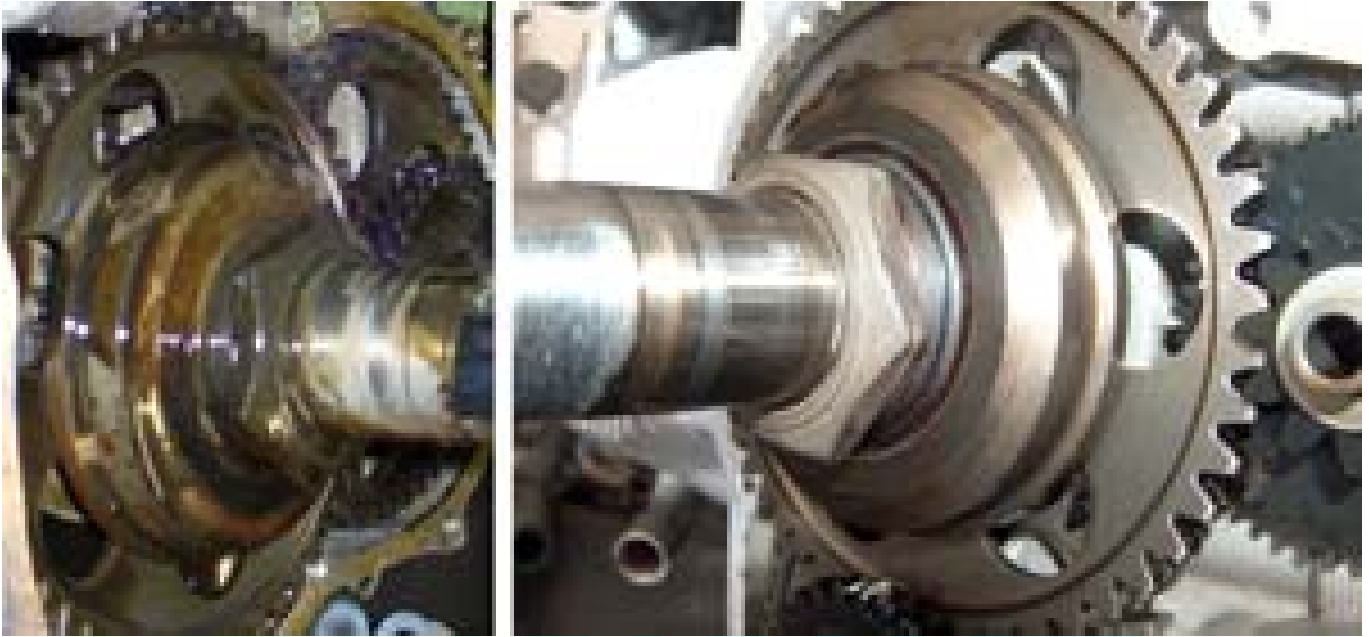
Figure 7: Sprag clutch in an engine run on Avgas (left) and the same component in an engine run on Unleaded Mogas
