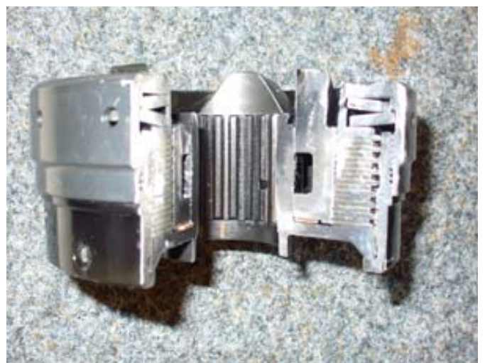
Figure 45: Cut away of slipper clutch
