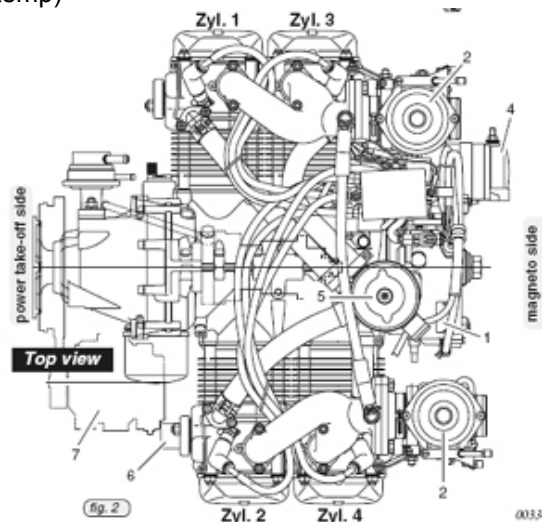
Figure 6: Drawing of cylinder orientation
