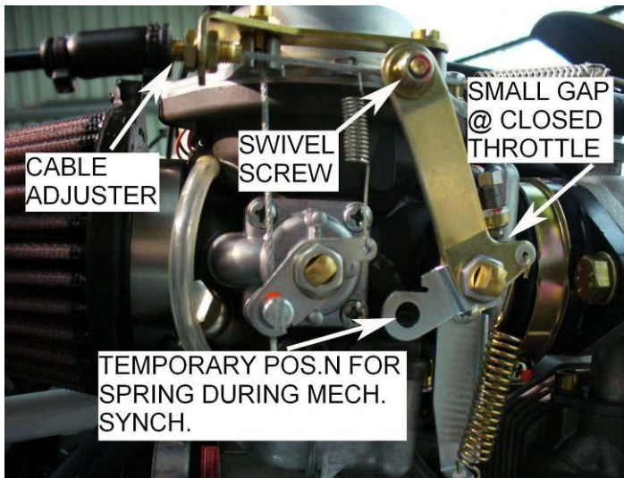
Figure 40a: Sprung open throttle system
