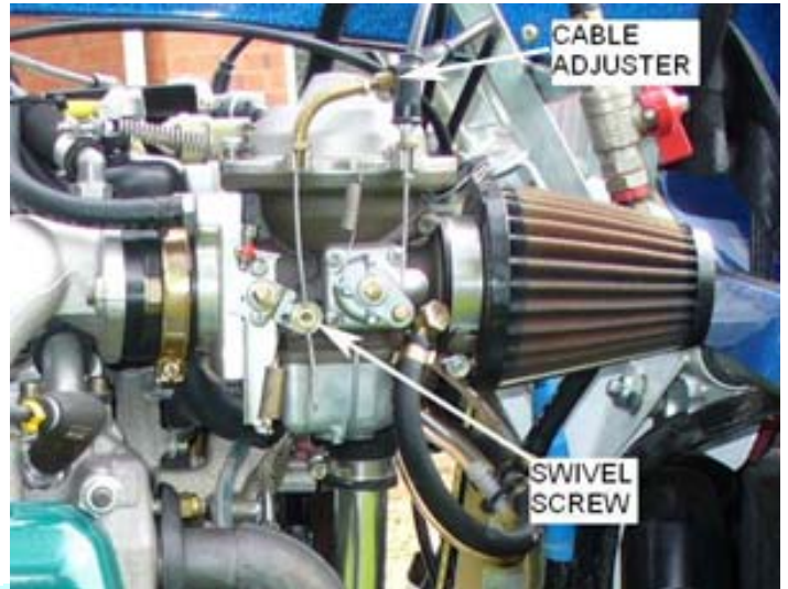
Figure 40b: Sprung closed throttle system
